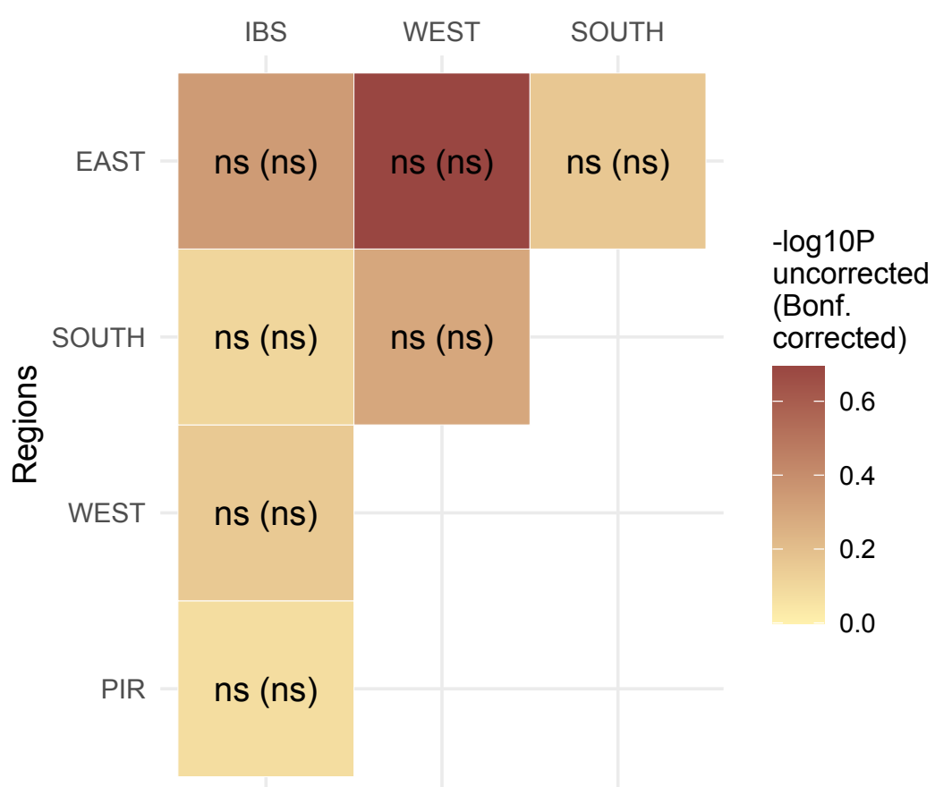
D Pairwise T-test of PRS among regions
